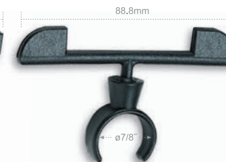
SW-412A Wider Price-card Holder (fit ø7/8" handlebar)
