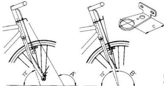
Basket back bracket for cantilever w. adjustable screw & nut set
